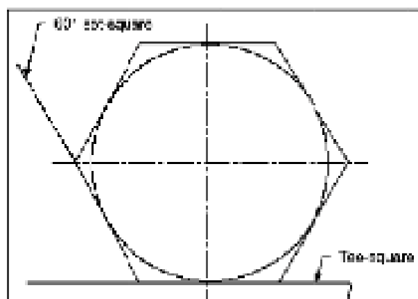
(c) Drawing a hexagon, given the distance across the flats.
