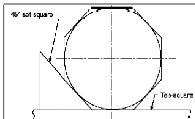
(e) Drawing a regular octagon, given the distance across the flats.
