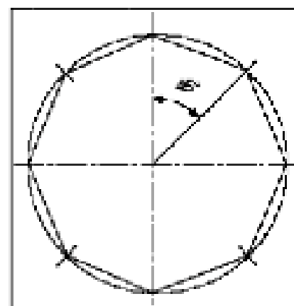
(d) Drawing a regular octagon, given the distance across corners.
