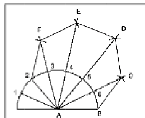
(f) Drawing a regular polygon, given the length of the sides.
